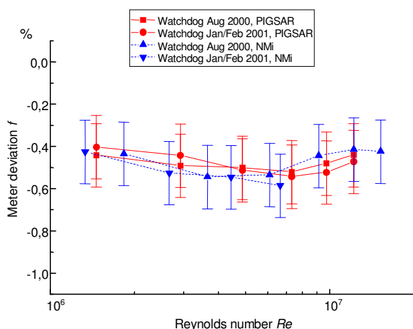
Fig. 12. - Calibration of a turbine meter DN250 (10'') as watchdog checks. The uncertainty level ( 2\sigma ) shown in the graph is the uncertainty U_{\text{Ref}} = 0,15\% of the harmonised reference value of PTB (Pigsar) and NMI-VSL as obtained in 1999. Compare with figure 2 to observe the effect of harmonisation: no bias is detectable for the end user any more.
