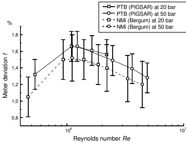
Fig. 2. - Typical results of meter calibration done at Pigsar and NMI-VSL (Bergum) before harmonisation (before 1999). All results of meter deviation f are inside the overlapping range of the uncertainty levels. Only due to high reproducibility of both calibration facilities as well as gas meters (which is much better than the uncertainties) a difference \Delta_{PTB-NMi} = f_{PTB} - f_{NMI} can be observed. The uncertainty levels ( 2\sigma ) shown in the graph are the particular uncertainties of Pigsar and NMI-VSL.
