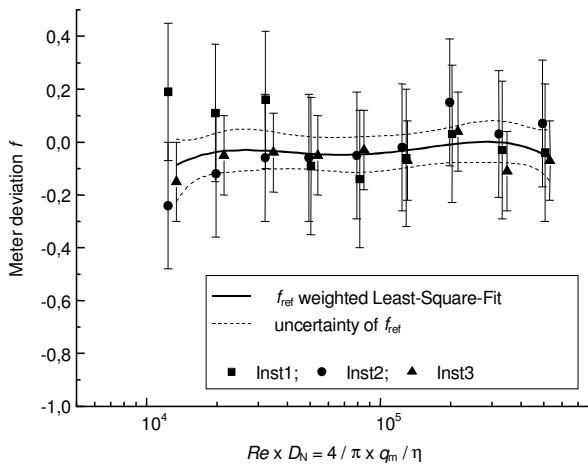
Fig. 8. - Practical measured meter deviations of one transfer meter within a package for one pressure . f_{\text{Ref}} is the weighted least-square-fit of all results (measured at 20 bar, package with two turbine meters, meter 1). This is the value that we use as the Harmonized European reference level.
