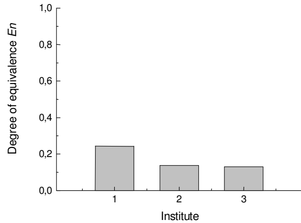
Fig. 11. - Characteristic degree of equivalence En for all institutes based on the geometric mean using all results in figure 10.
