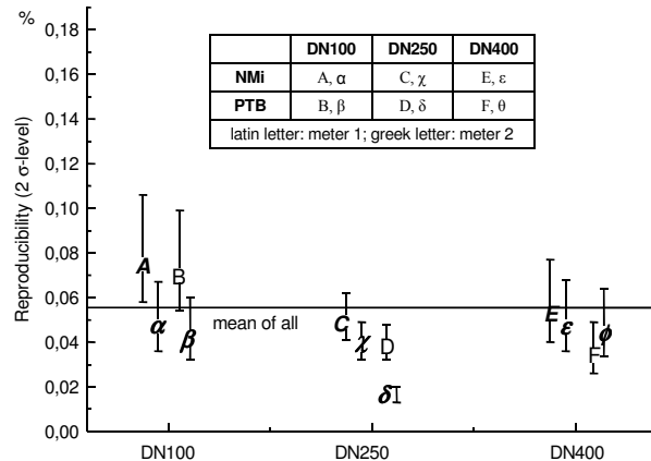
Fig. 6. - Results of reproducibility calculation for all transfer meters used in harmonization between NMI-VSL (Netherlands) and PTB (Germany). The calculation is based on all measurement within 1999 to 2003.
