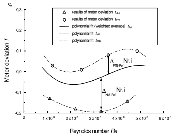
Fig. 3. - Results of comparison for one meter at one pressure stage and determination of differences \Delta_{PTB-Ref} and \Delta_{NMI-Ref} .
