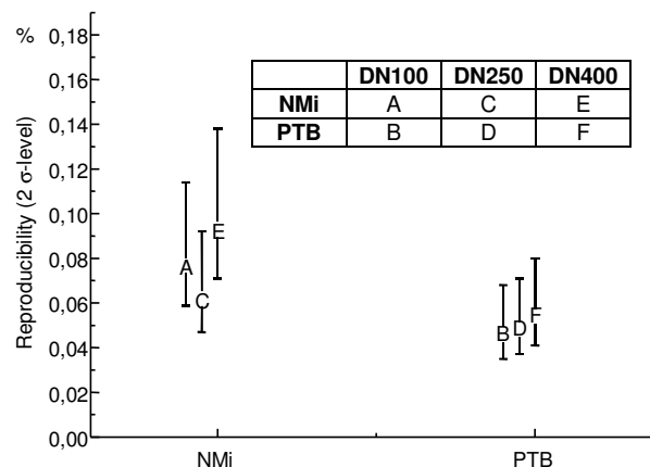
Fig. 7. - Results of reproducibility calculation for the facilities of NMI (Netherlands) and PTB (Germany) within the harmonization. The calculation is based on all measurement from 1999 to 2003.
