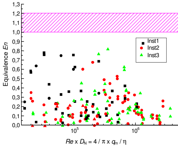
Fig. 10. - Degrees of equivalence En determined for all results determined at all high press national facilities in Europe, namely PTB-Pigsar, NMI-VSL and LADG [Measured at 20 bar; 40 bar and 50 bar; packages (DN150, DN250, DN400) with two turbines each; additionally single sonic nozzle (TF200)].
