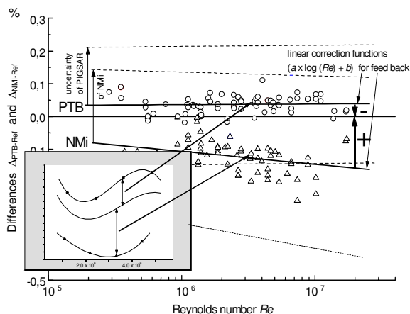
Fig. 4. - Summary of all determined differences \Delta_{PTB-Ref} and \Delta_{NMI-Ref} for all meters in all pressure stages plotted as function of the Re -number.
