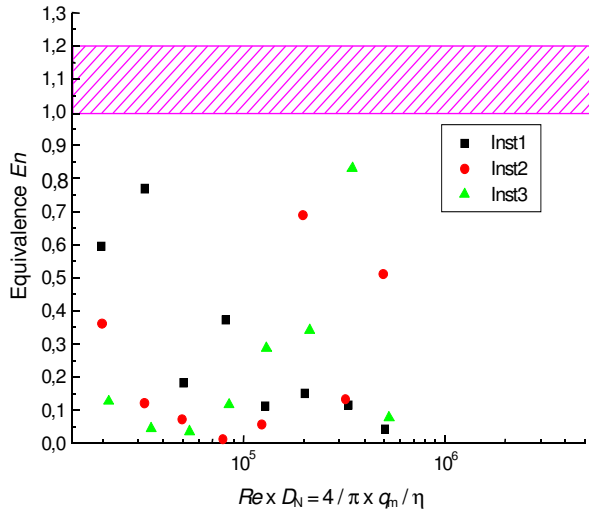
Fig. 9. - Degrees of equivalence En determined for all measured results in figure 8.
