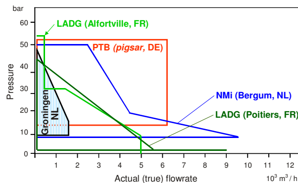
Fig. 1. - Calibration and measuring capabilities of PTB-Pigsar, NMI-VSL and LADG. Harmonization has been mainly applied in the overlapping ranges.
